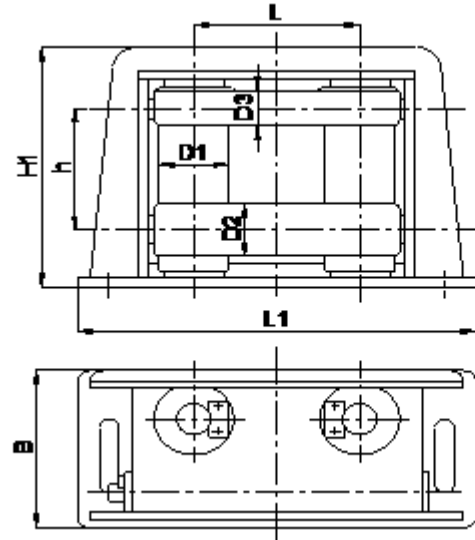
JIS F-2026 HORIZONTAL FAIRLEAD ROLLER TYPE A 4 ROLLERS
